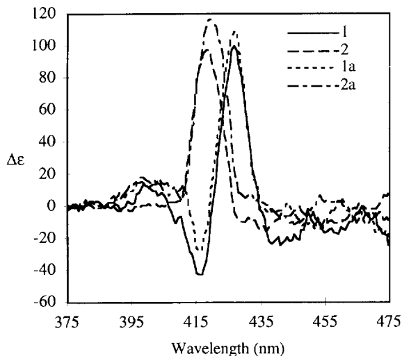
Figure 2. Circular Dichroism Spectra of Dimers
